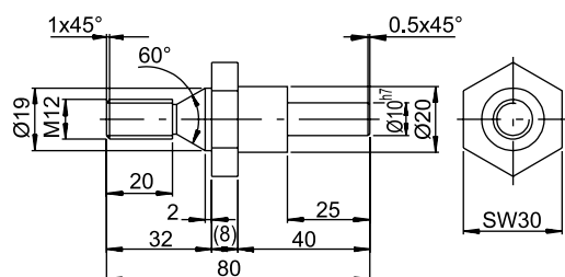
Wellenadapter M12
