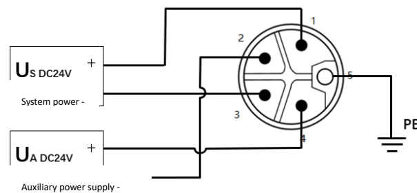
Power port
