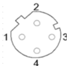
M12,D-Coded,Female
