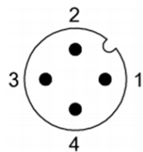
M12,A-Coded,Male
